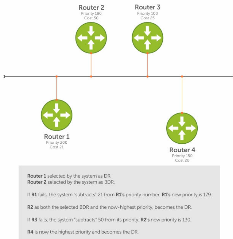
Figure 92. Priority and Cost Examples
